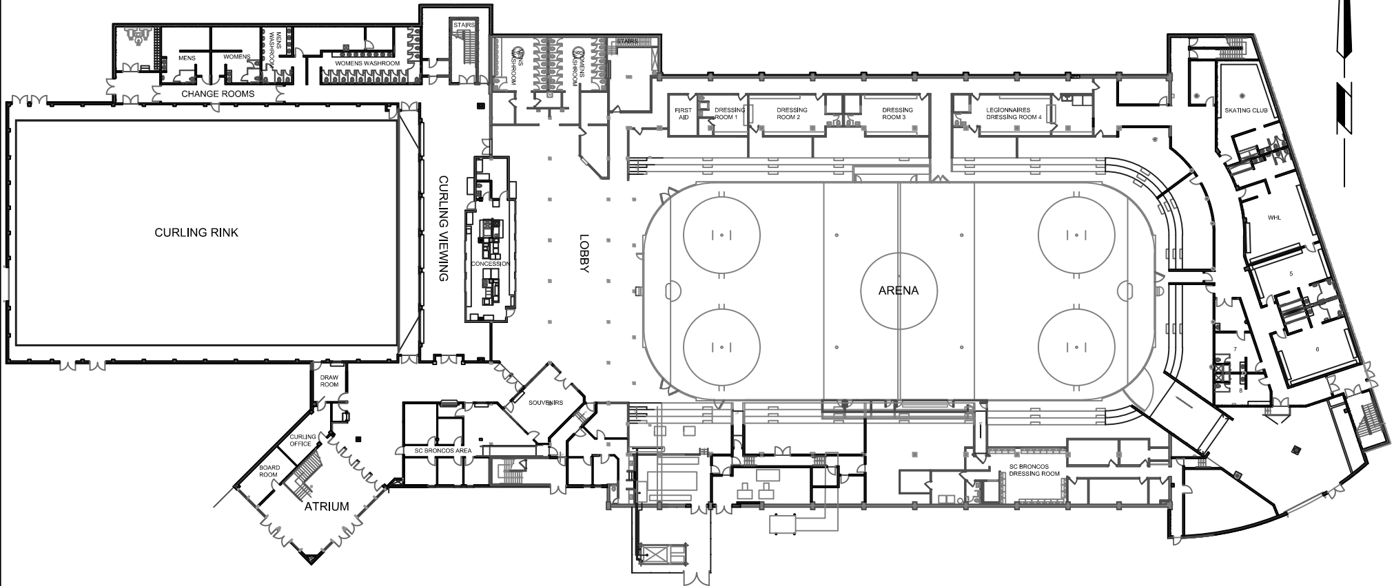
MAIN LEVEL LAYOUT
